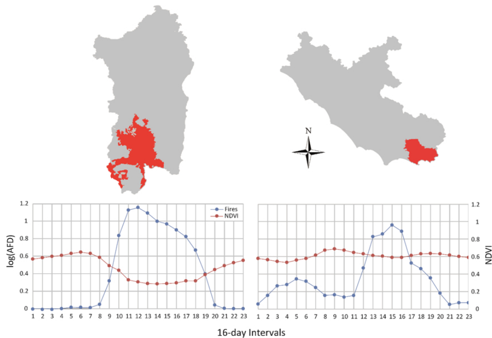
Figure 2. Location of the fire hot spots of Sardinia and Latium with the corresponding pyrophenological diagrams. The 16-day intervals used for constructing the diagrams are: 1–16 Jan (1), 17 Jan–1 Feb (2), 2–17 Feb (3), 18 Feb–5 Mar (4), 6–21 Mar (5), 22 Mar–6 Apr (6), 7–22 Apr (7), 23 Apr–8 May (8), 9–24 May (9), 25 May–9 June (10), 10–25 Jun (11), 26 Jun–11 Jul (12), 12–27 Jul (13), 28 Jul–12 Aug (14), 13–28 Aug (15), 29 Aug–13 Sept (16), 14–29 Sept (17), 30 Sept–15 Oct (18), 16 Oct–31 Oct (19), 1–16 Nov (20), 17 Nov–2 Dec (21), 3–18 Dec (22), 19–31 Dec (23).
